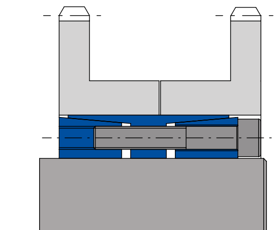
Simultaneously locking two sprockets using SEL4500.
