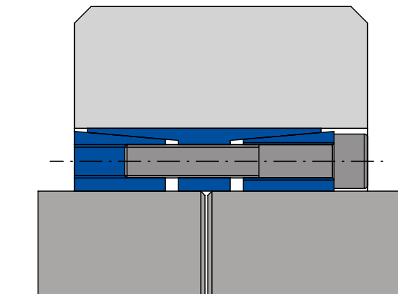
Locking two shafts and a hub using SEL4500. Only one locking device is used for locking 3 components.
