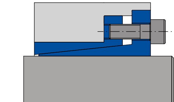
SEL1100 hub applications without spacer. Recommended for high rotation speeds.
