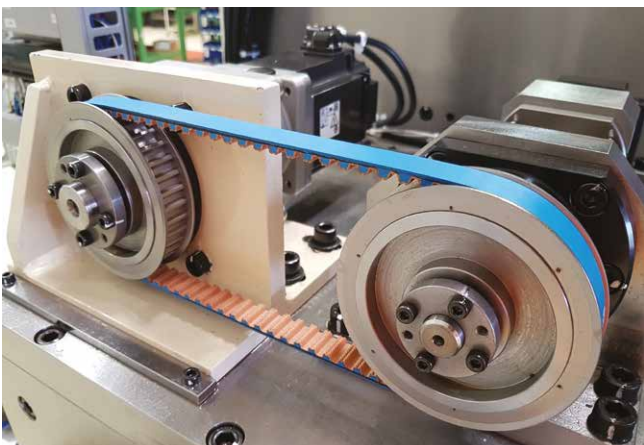
Mounting two pulleys using SEL1100 without spacers.
