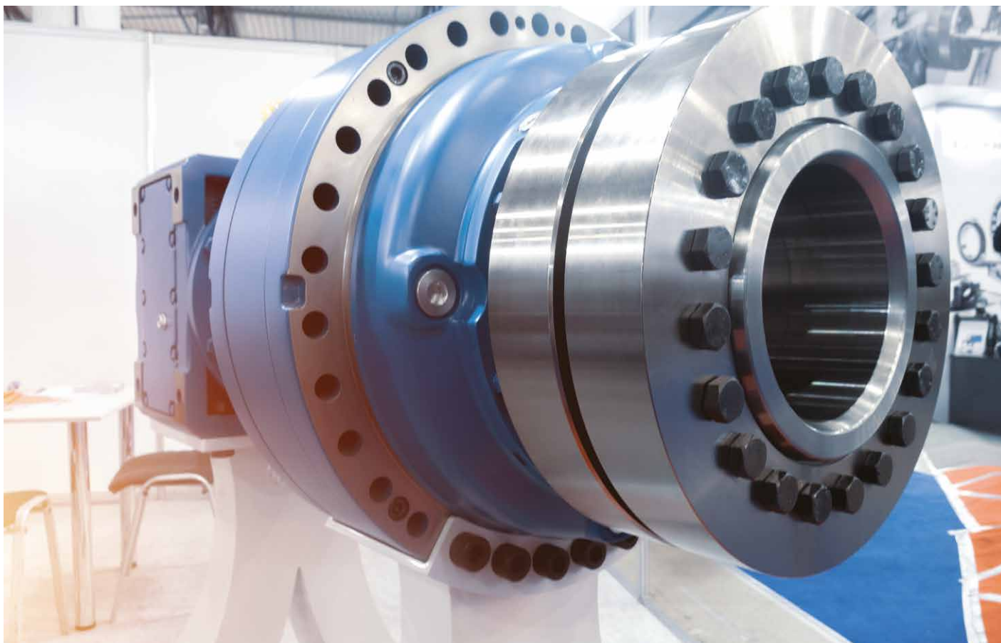
Locking the hollow shaft of a planetary gearset using SEL6030.
