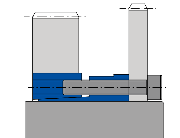
Joining a timing belt pulley and a brake disc with SEL1300.
