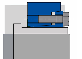
SEL6210, SEL6220, SEL6230, SEL6810, SEL6830 not assembled
