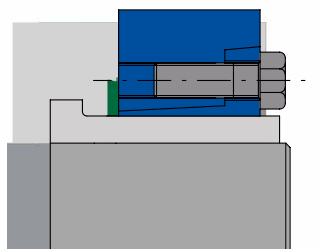
SEL6210, SEL6220, SEL6230, SEL6810, SEL6830 assembled
